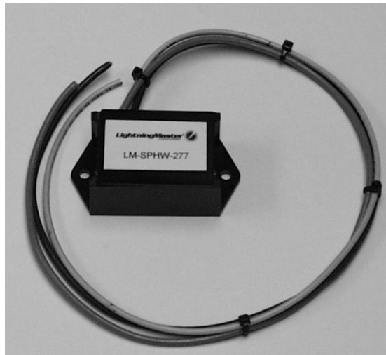
Hard-wired single phase surge suppressor - 120V
