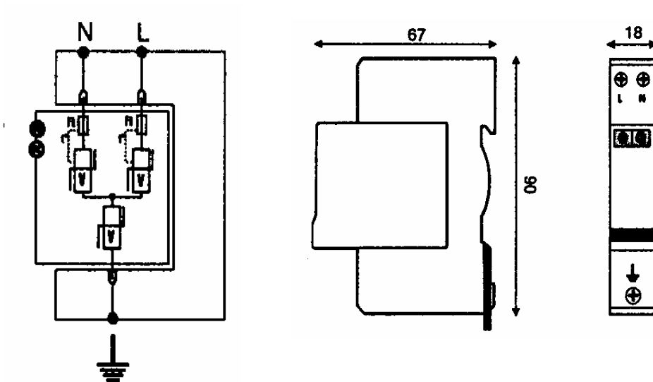
D.I.N Rail 17.5" Steel
