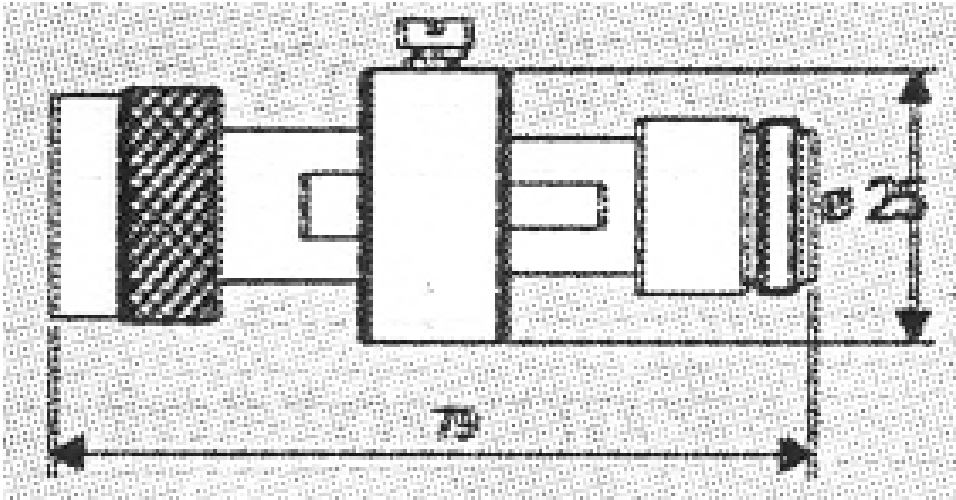
Coaxial Cable Surge Protector – N Connectors.
