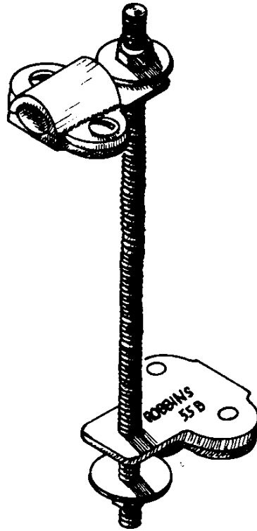
Thru Wall Cable Connector 1/2" Rod Copper
