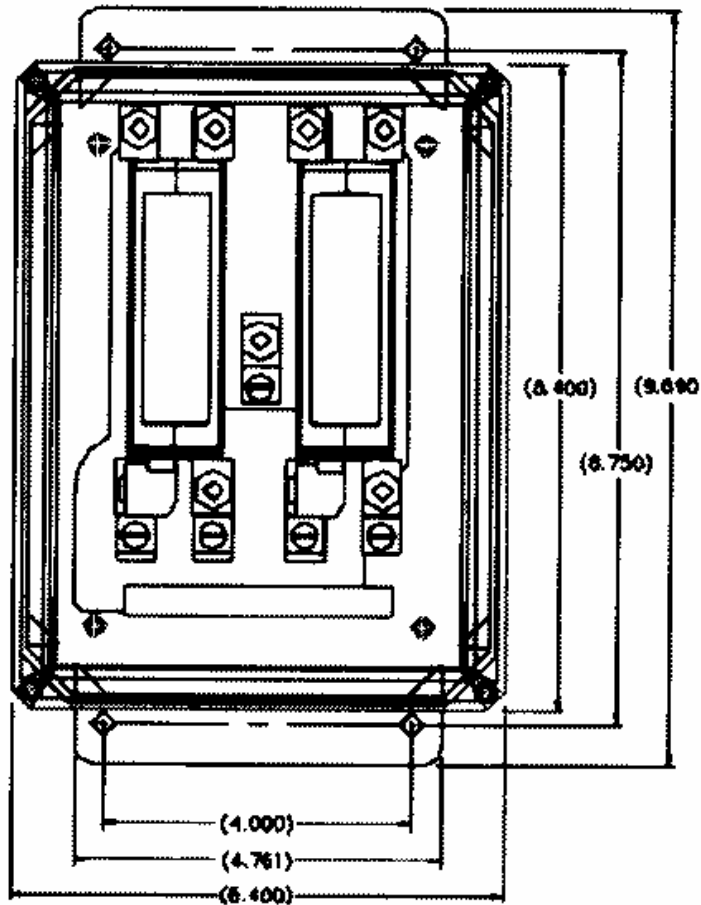
LM-480V, 3 phase, Main
