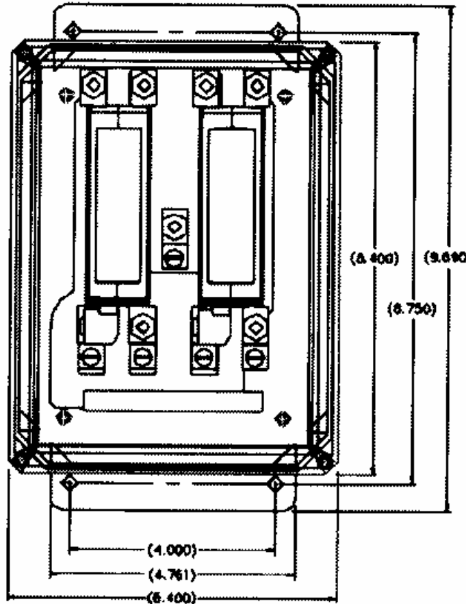
LM-240/415V, 3 phase, Main
